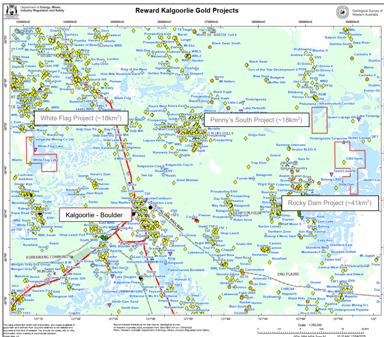
Figure 6 – Reward's Kalgoorlie Gold Projects shown with Geological Survey of Western Australia known gold occurrences; White Flag (E24/243 – ~18km 2 ), Penny's South (E27/736 - ~18km 2 ) and Rocky Dam (E25/655 - ~41km 2 ).
