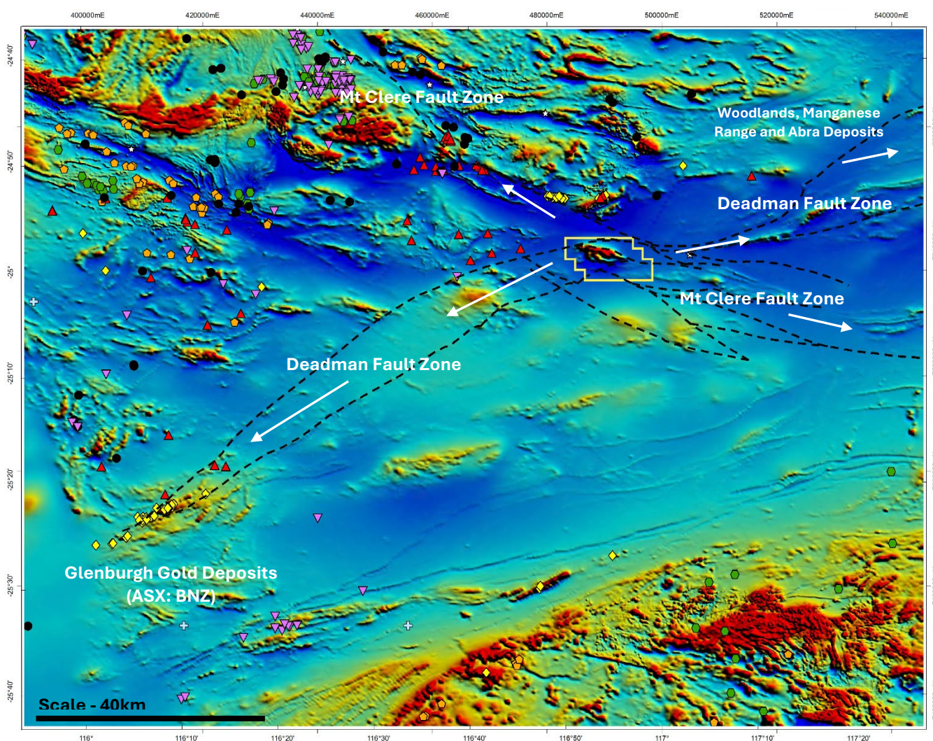
Figure 5 – Exploration Licence application E52/4510, shown with a regional magnetic image, major structures thought to control mineralisation and known mineral occurrences; yellow diamonds (gold) and red triangles (base metals) -Source: Geological Survey of Western Australia Geoview website.
