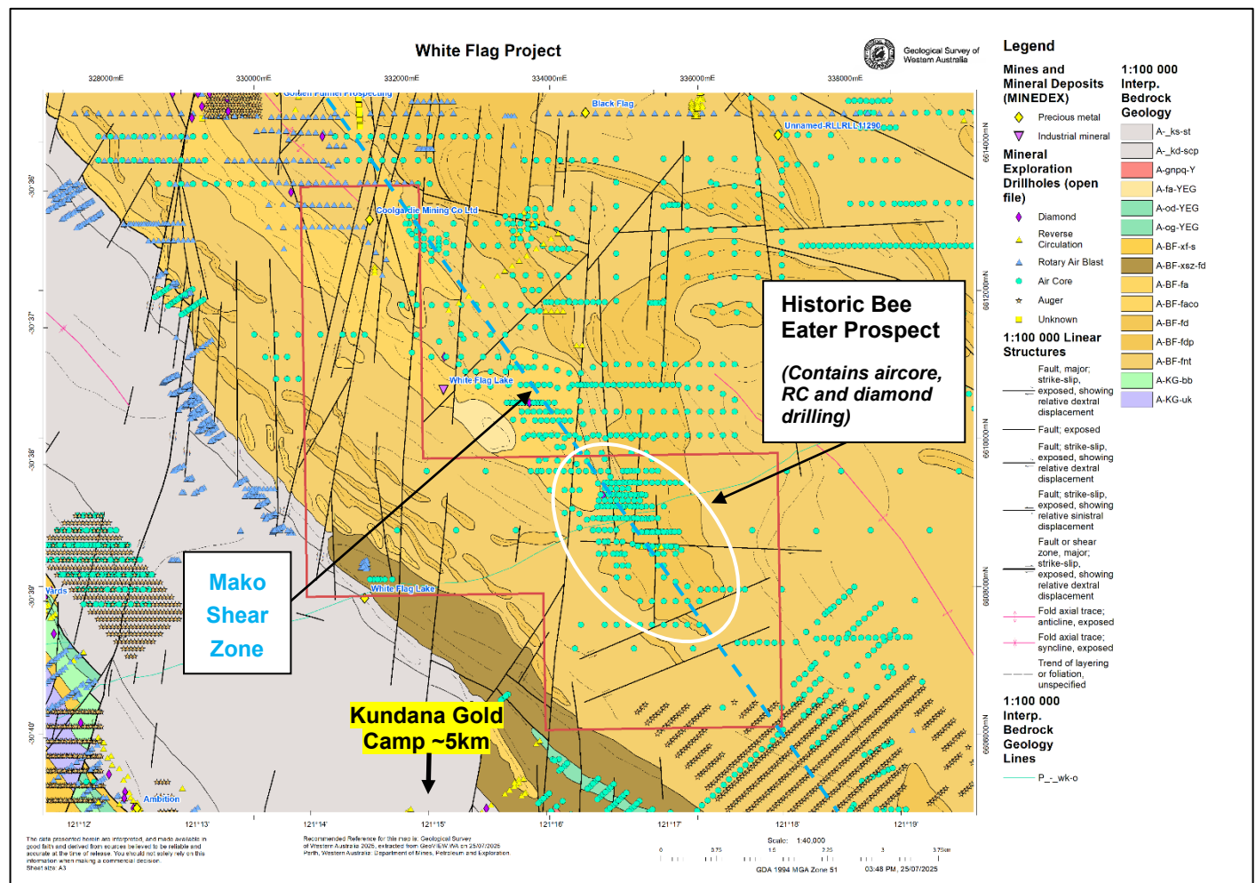
Figure 7 – The White Flag Project (E24/243) at 1:40,000 scale over Geological Survey of WA (GSWA) 1:100,000 scale Interpreted Bedrock Geology Map showing historical drill collar locations extracted from the GSWA Geoview Website. The Bee Eater Prospect has received the most historic exploration including ground-based geophysics, aircore, RC and diamond drilling completed by Delta Gold, Placer Dome Asia Pacific and Barrick 1 (further detailed information from the historic exploration activities will be provided once data compilation activities are suitably advanced).
