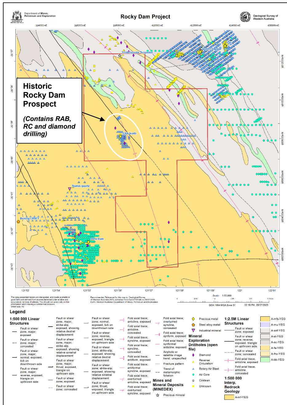
Figure 8 – The Rocky Dam Project (E25/655) at 1:50,000 scale over Geological Survey of WA (GSWA) 1:500,000 scale Interpreted Bedrock Geology Map showing historical drill collar locations extracted from the GSWA Geoview Website. The CRA-NTH Prospect has received the most historic exploration including airborne geophysics, geological mapping, RAB, RC and diamond drilling completed by CRA, North, Dreadnought Resources and Lycaon 1 (further information from the historic exploration activities will be provided once data compilation activities are suitably advanced).
